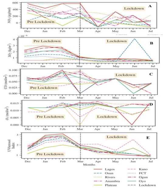
Figure 2. Time series of monthly averages of NO 2 , SO 2 , CO, O 3 , and UV Aerosol concentration between Dec 2019 and July 2020
