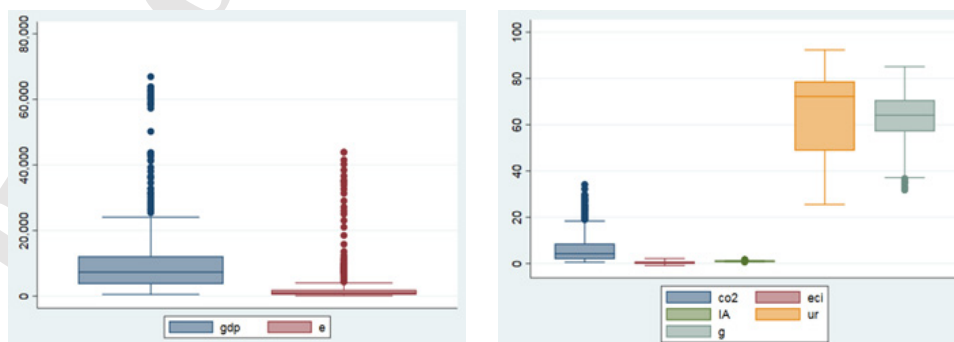
Fig 2. Box plot of research variables
