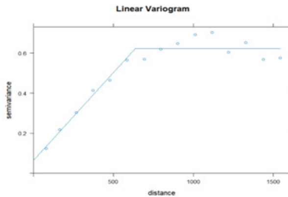
Fig. 6 Linear Semivariogram model fitting
