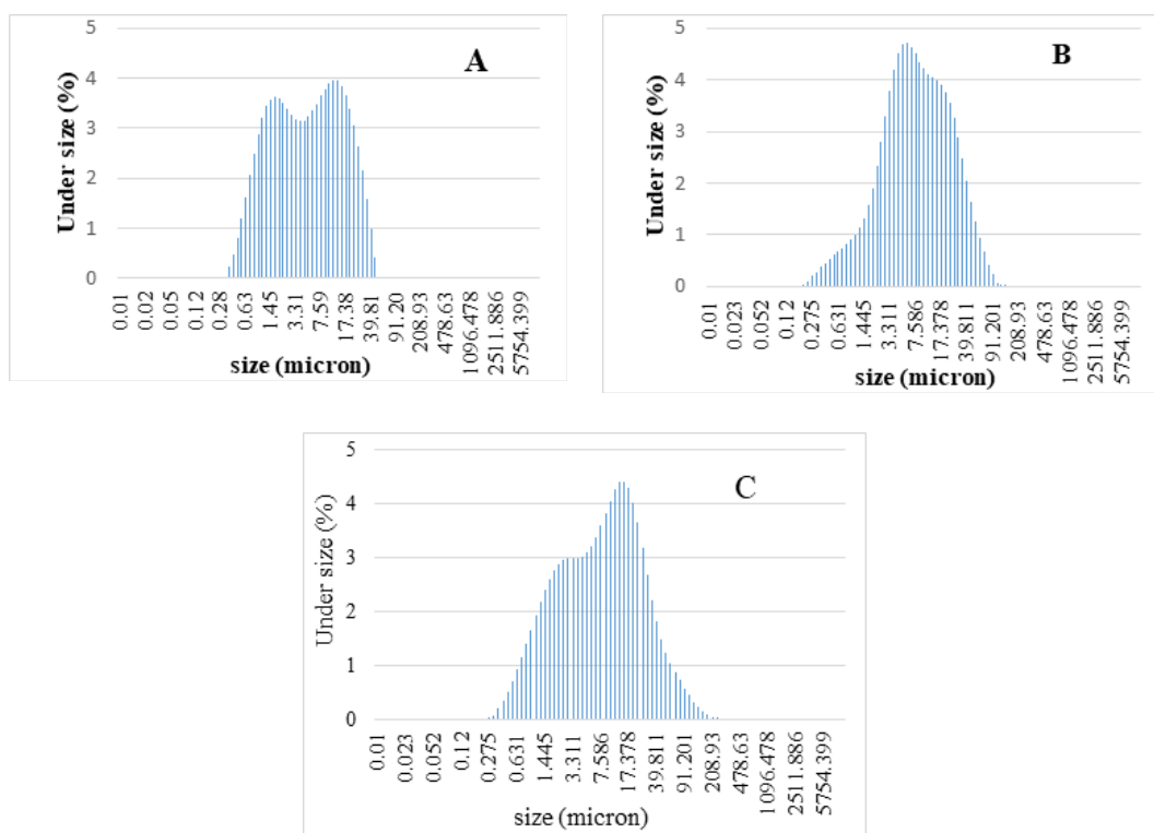
Figure 7: Particle size distribution diagram of mechanically activated phosphate concentrate at Ball to powder ration of 20:1, dry milling, argon atmosphere, balls diameter of 9.4 mm, rotation speed of 500 rpm and activation time of; A) 20 min, B) 60 min, C) 90 min
